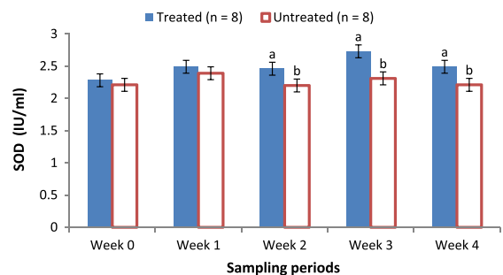
Fig. 1. Changes in superoxide dismutase (SOD) activity in horses administered with or without resveratrol. Values with different letters are significantly different ( P < .05 ).
