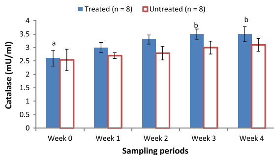
Fig. 3. Alterations in catalase activity in horses administered with or without resveratrol (mU/mL). Values with different letters are significantly different ( P < .05 ).
