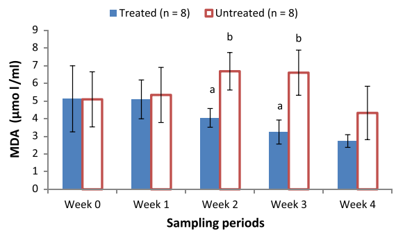
Fig. 4. Changes in malondialdehyde (MDA) concentration in horses administered with or without resveratrol ( \mu\text{mol/mL} ). Values with different letters are significantly different ( P < .05 ).
