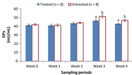
Fig. 2. Variations in glutathione peroxidase (GPx) activity in horses administered with or without resveratrol (mU/mL). Values with different letters are significantly different ( P < .05 ).
